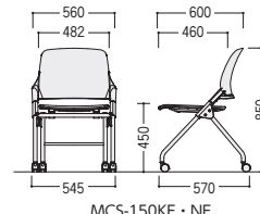
MCS-150KF・NF
