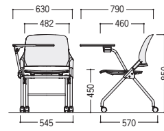
MCS-150MKF・MNF
